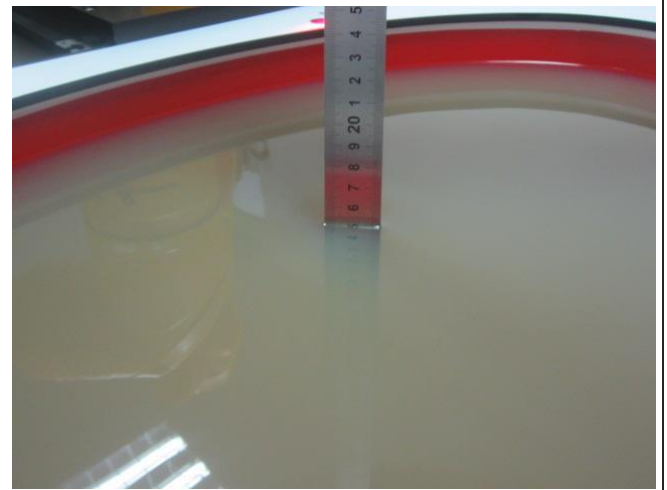
Liquid depth in the ELI phantom(Limbs)
