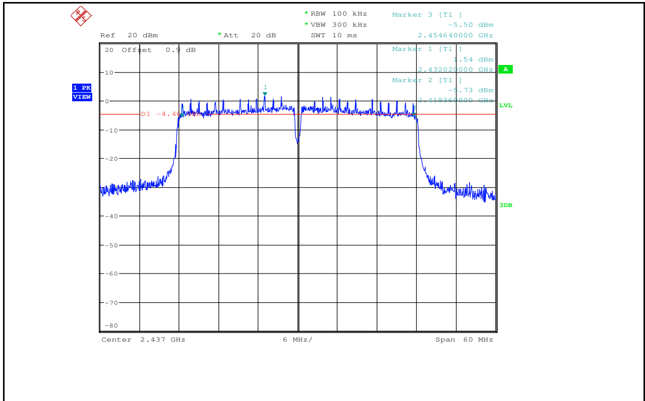
6dB Bandwidth_11N40SISO_2437_Ant2
