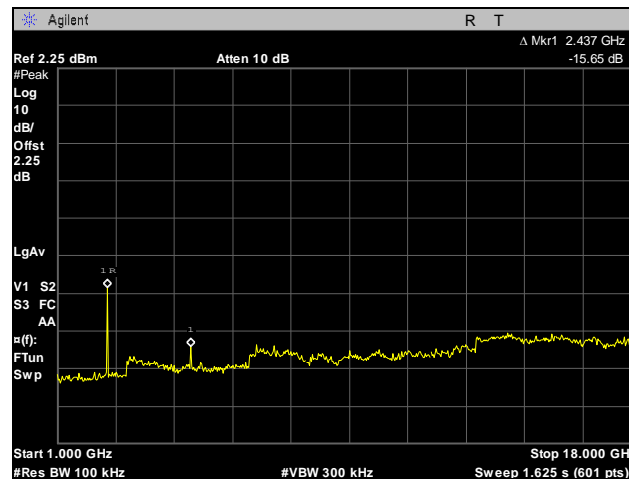
Plot 25. Conducted Spurious Emissions, Mid Channel, 1 GHz – 18 GHz
