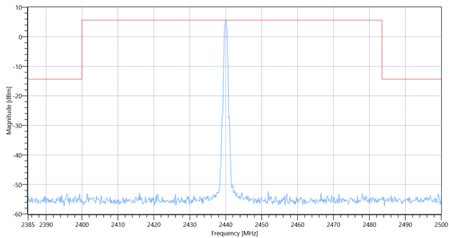
FCC 15.247 # TX spurious conducted 20dBc ~ BT LE 1 Msp 2440
