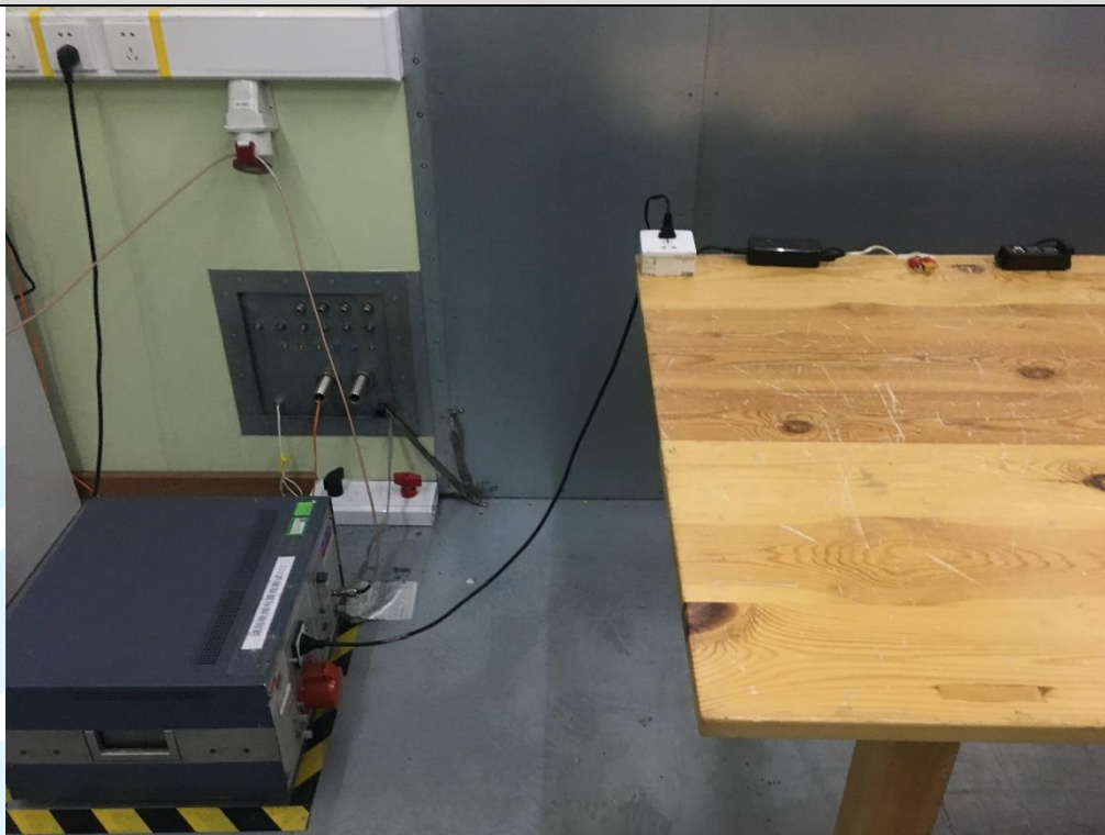
Conducted Emission Test Setup - Mode 2
