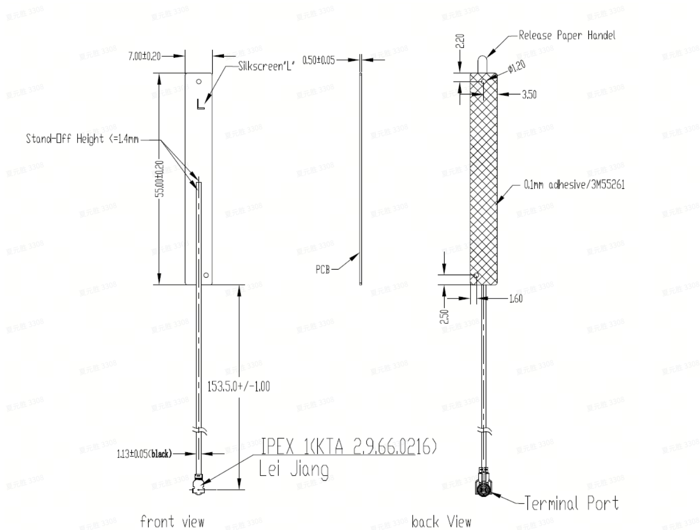
Right Antenna
