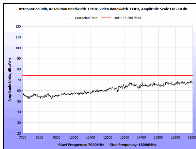
Plot 19. Radiated Spurious Emissions, High Channel, 7 GHz – 18 GHz, Peak
