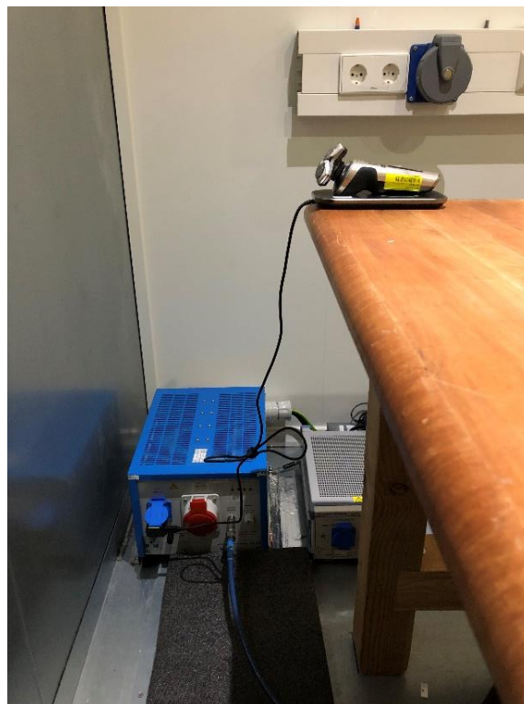
4. Conducted Emission test setup
