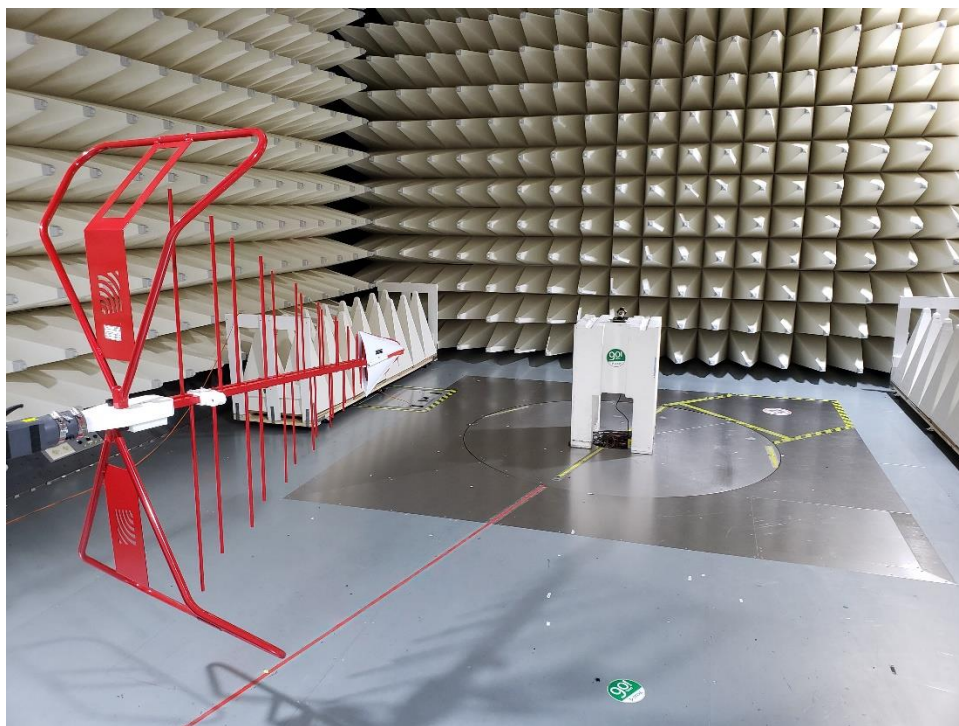
6. Low Range Radiated Emission test setup (30MHz to 1GHz)
