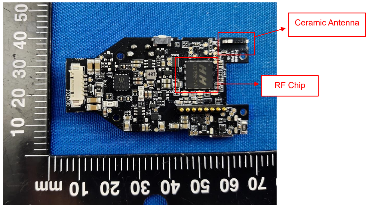
MAIN BOARD REAR VIEW
