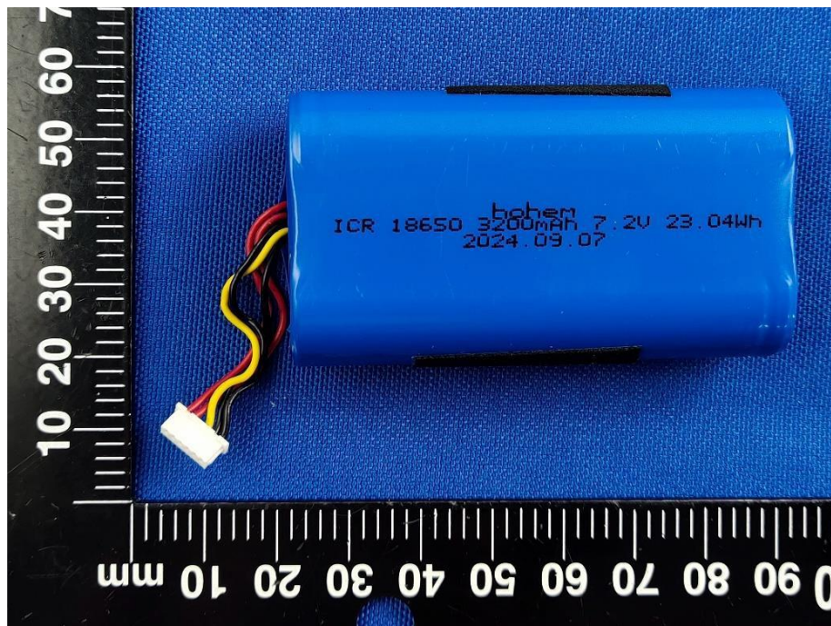
BATTERY (FRONT)
