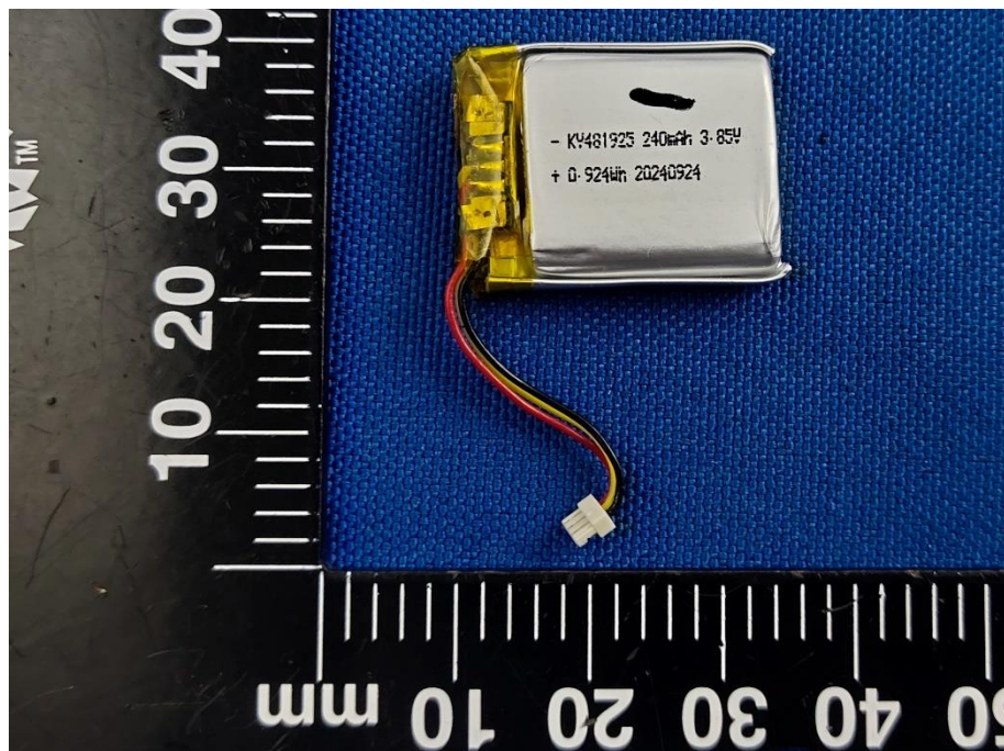
BATTERY (FRONT)
