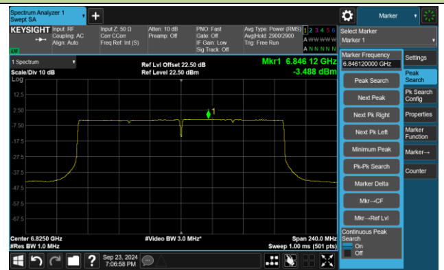
Channel 175 (6825MHz)
