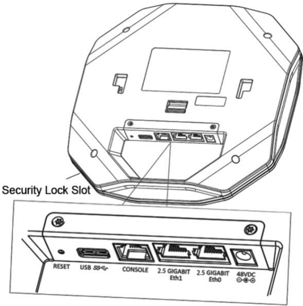
Figure 3: OAW-AP1431 Back View
