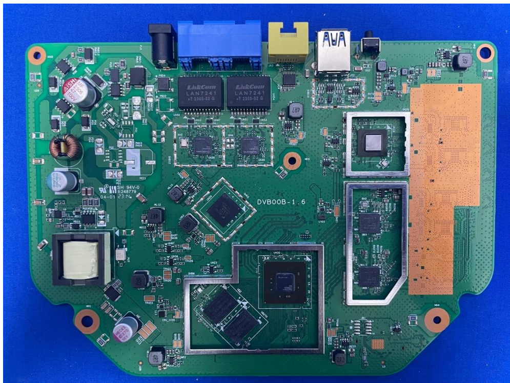
(16) EUT Photo (OAW-AP1411)
