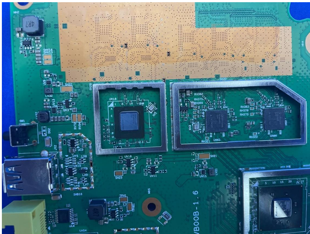
(20) EUT Photo (OAW-AP1411)
