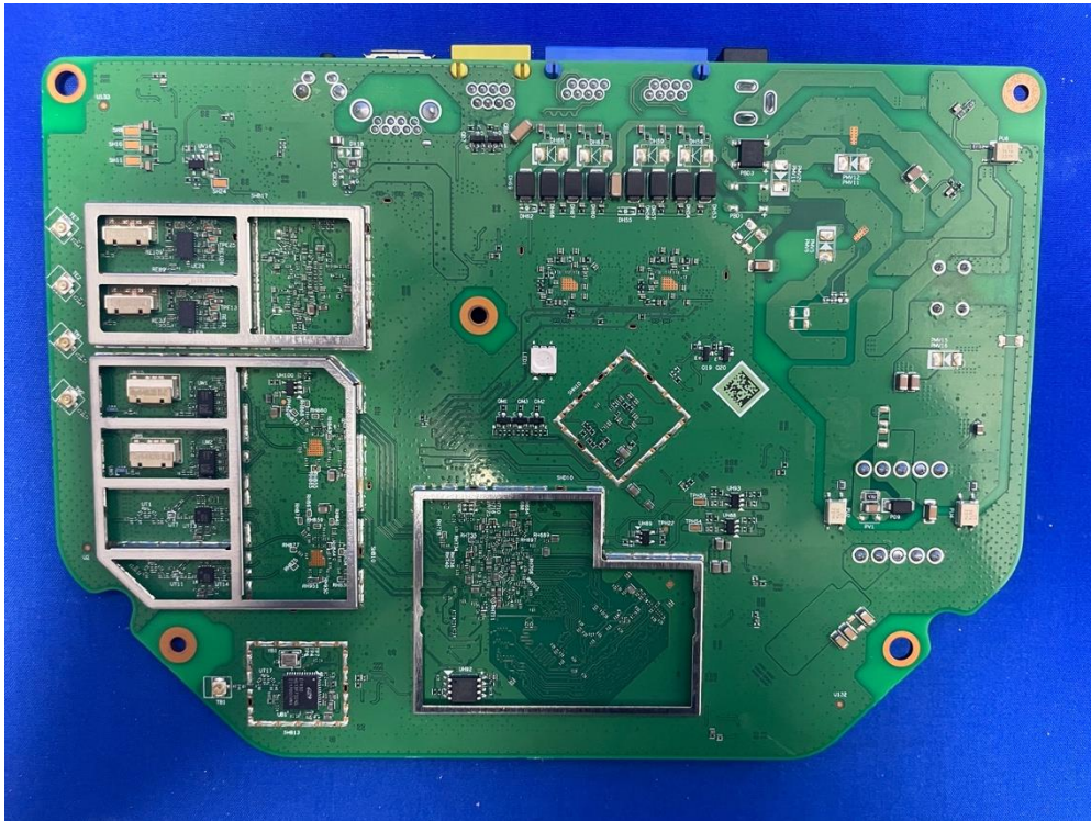
(21) EUT Photo (OAW-AP1411)
