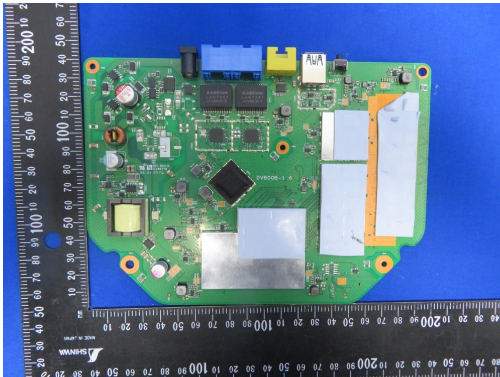
(15) EUT Photo (OAW-AP1411)
