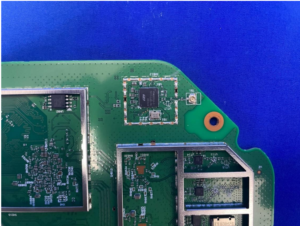
(11) EUT Photo (OAW-AP1431)
