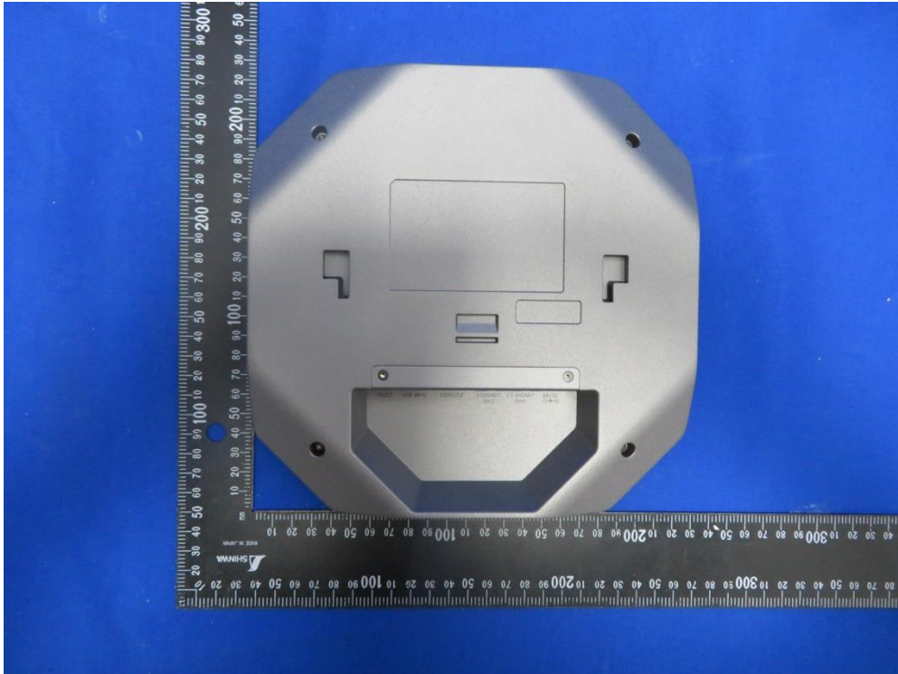
(9) EUT Photo (OAW-AP1411)
