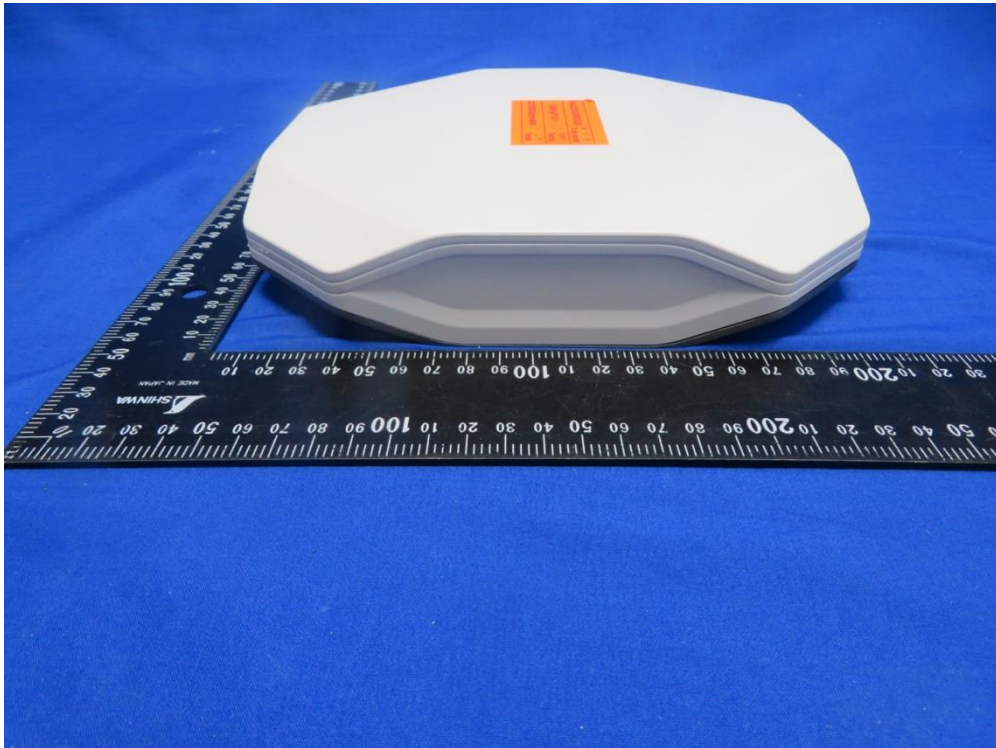
(7) EUT Photo (OAW-AP1431)
