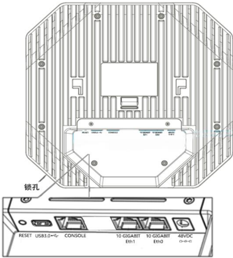
Figure 3: OAW-AP1351 Back View
