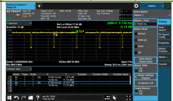
802.11ax-HE20 (T = 5.430ms)
