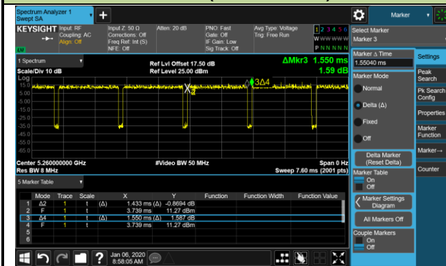
802.11n-HT40 (T = 5.400ms)
