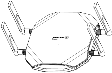
Figure 5: Install the external antenna on OAW-AP1322.
