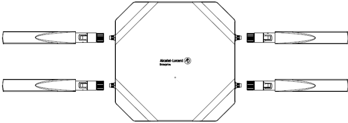
Figure 5: Install the external antenna on OAW-AP1322.
