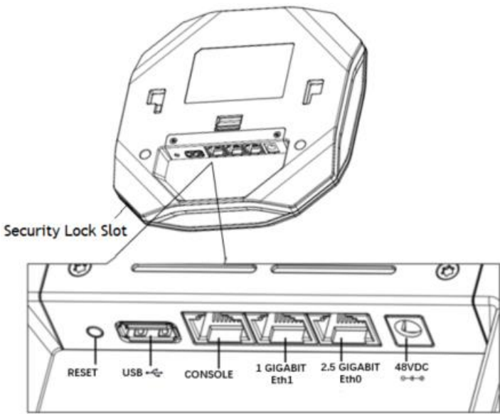
Figure 6: OAW-AP1320 Series Back View
