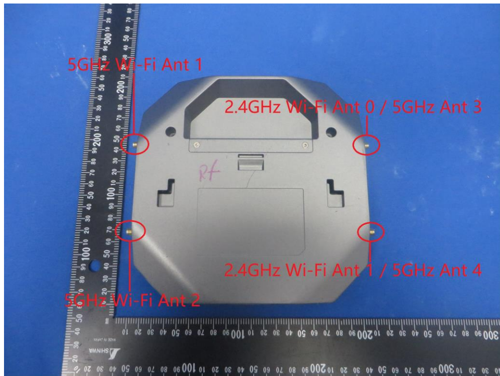
(5) EUT Photo_OAW-AP1322
