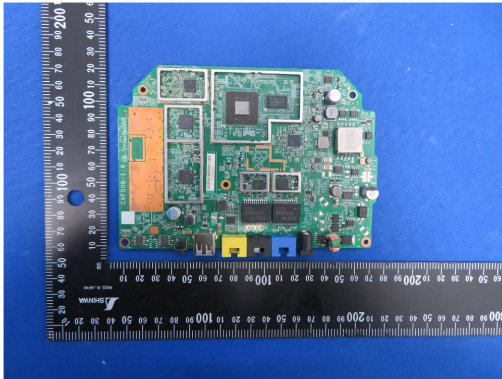
(11) EUT Photo_OAW-AP1322
