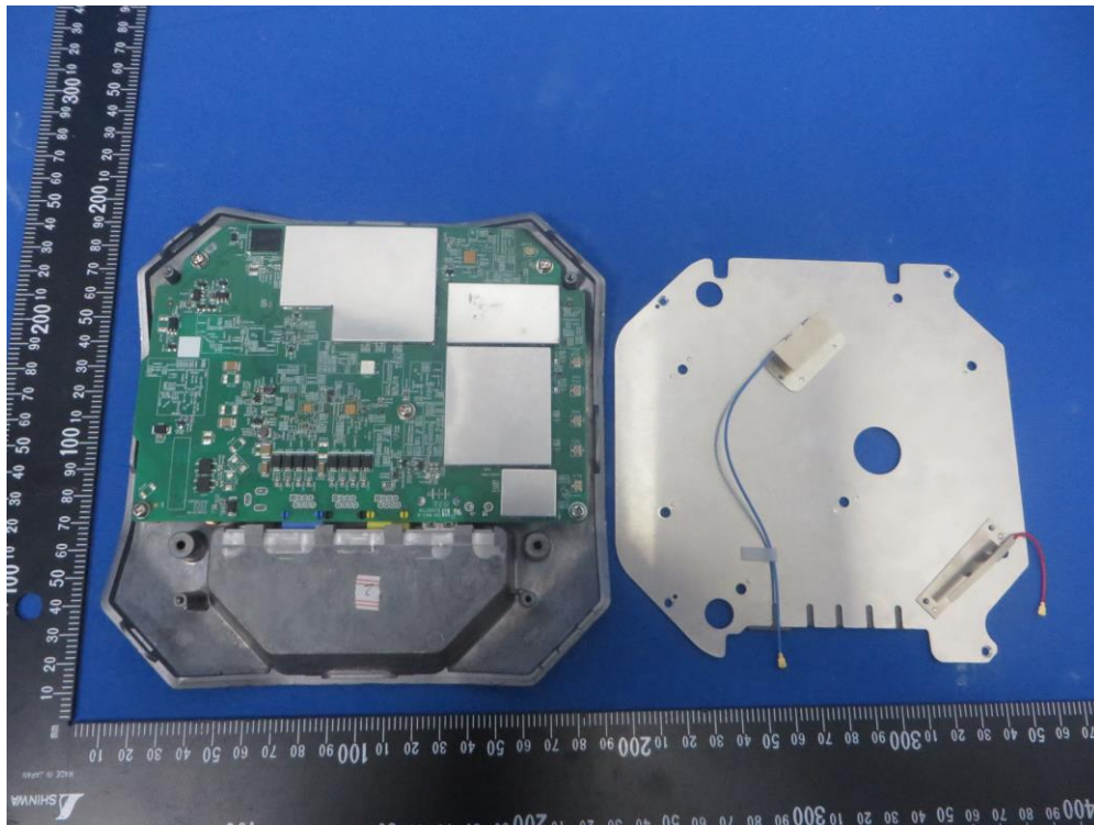
(9) EUT Photo_OAW-AP1322
