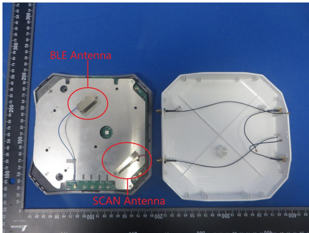
(8) EUT Photo_OAW-AP1322
