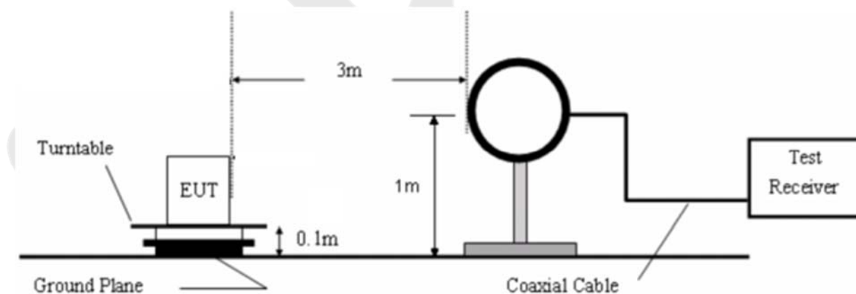
Figure 1. Below 30MHz
