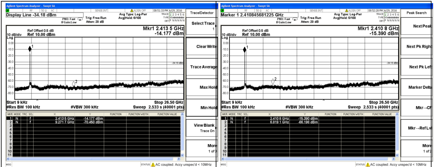
802.11n-HT20-Low Channel, 2412MHz
