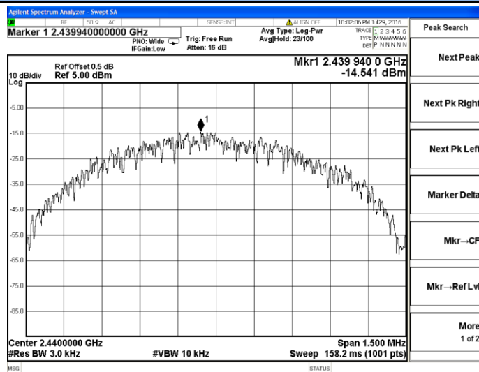
BT LE-Middle Channel, 2440MHz
