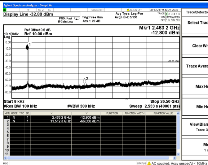
802.11n-HT20-High Channel, 2462MHz
