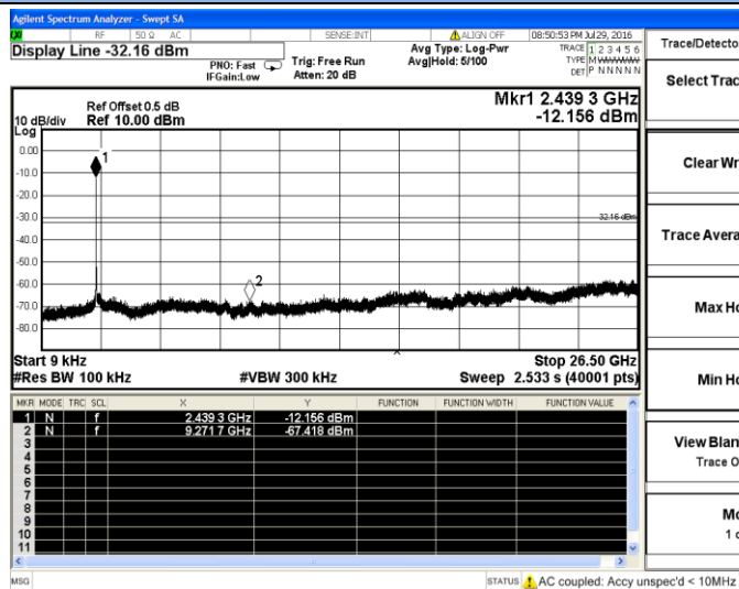
802.11n-HT20-Middle Channel, 2437MHz
