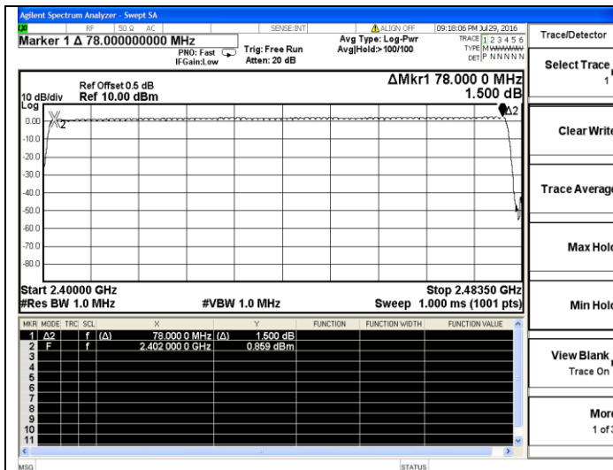
Test Plot For Number of Hopping Channel(GFSK)
