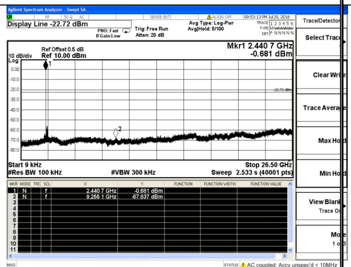
9KHz-26.5GHz Middle Channel(GFSK)
