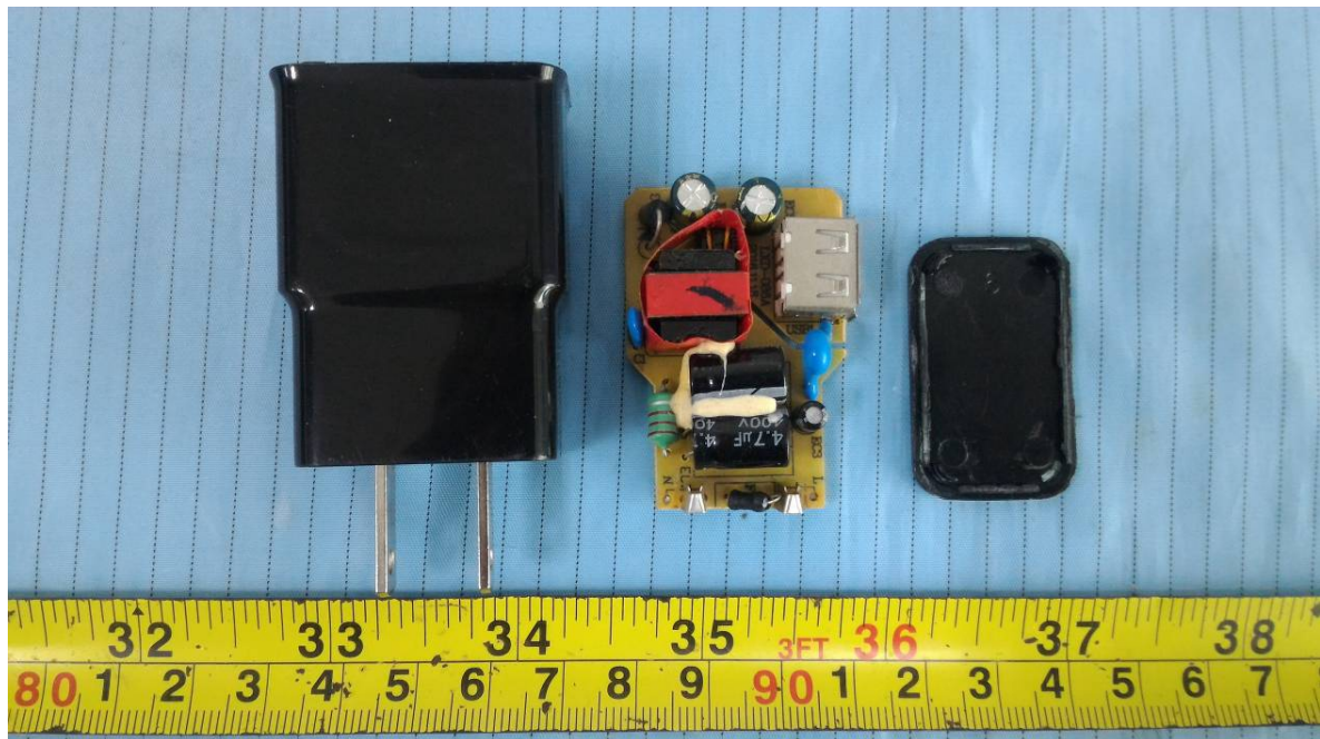
EUT – Adapter Cover off View
