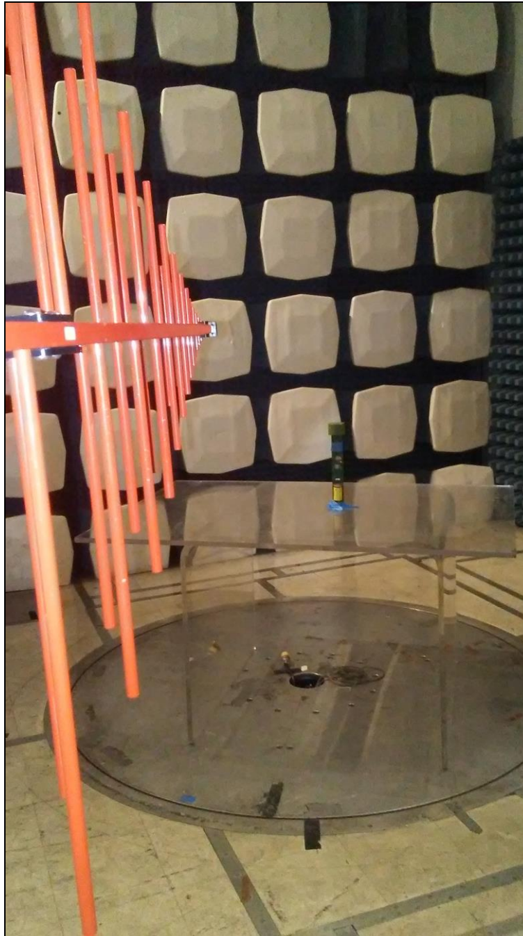
Photograph 1. Radiated Spurious Emissions Setup, Below 1GHz
