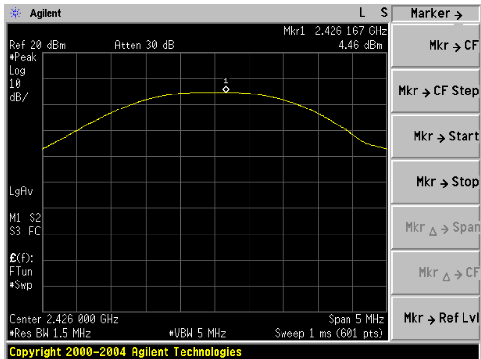
Peak output Power plot on channel 38
