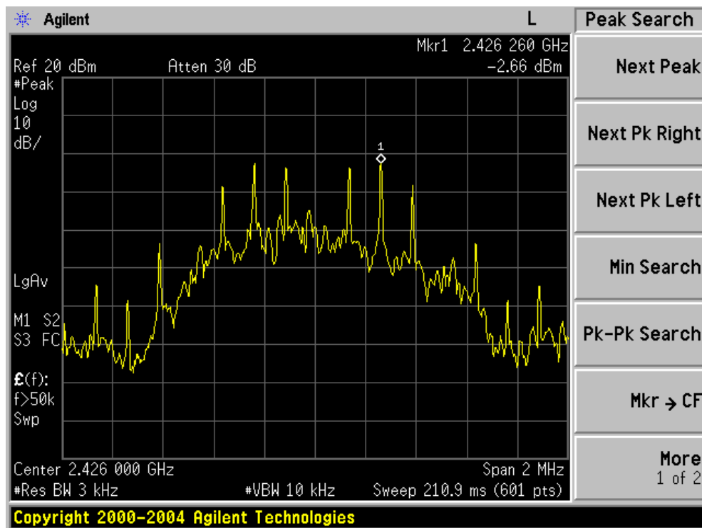
Power spectral density plot on channel 38
