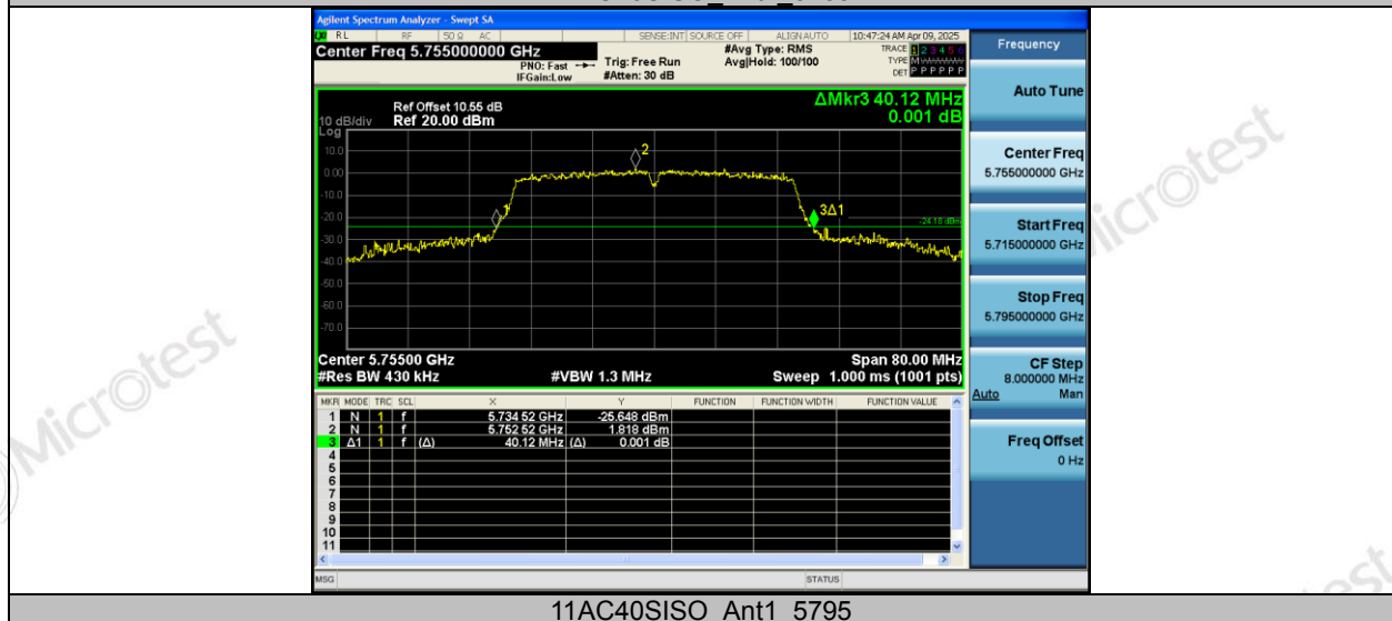
11AC40SISO_Ant2_5755
