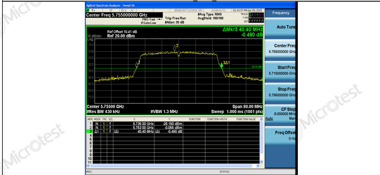
11AC40SISO_Ant2_5755
