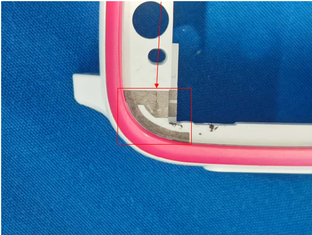
WIFI Antenna
