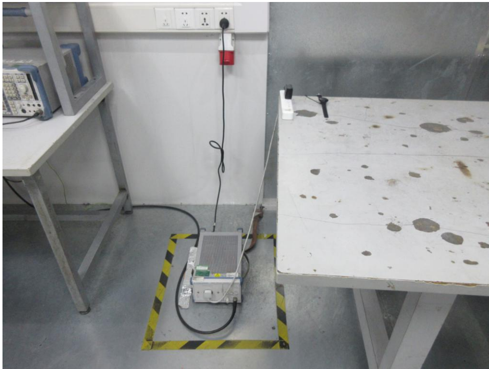
FCC ID: 2A16I-H1118 Photo of Power Line Conducted Emission Test
