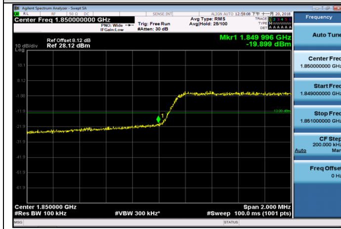
LCH_QPSK_15RB#0
