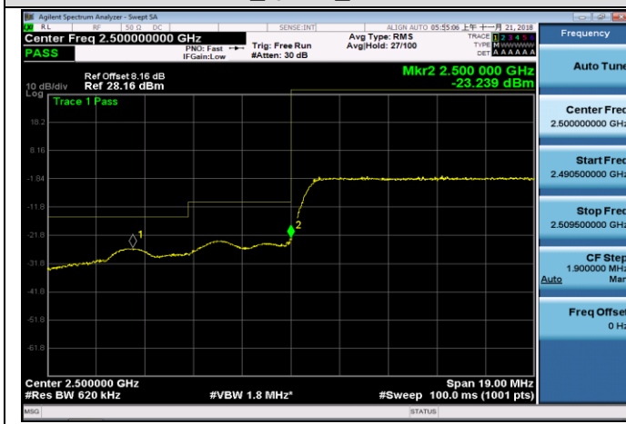
LCH_QPSK_75RB#0
