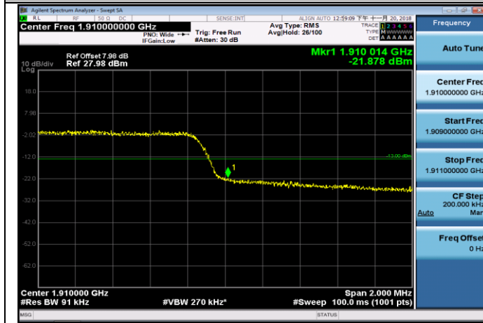
HCH_QPSK_15RB#0
