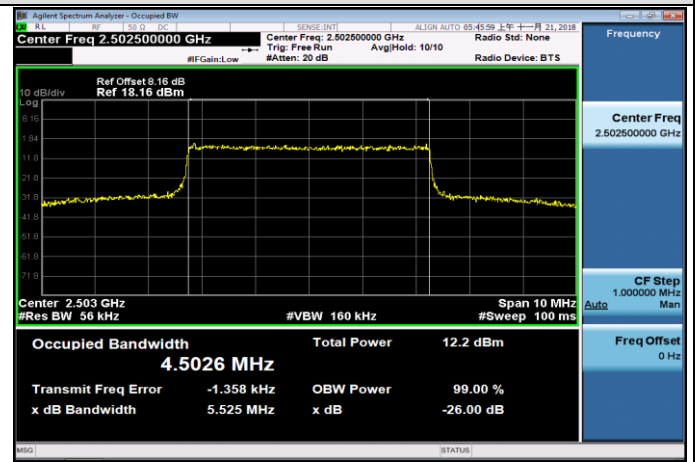
LCH_16QAM_25RB#0
