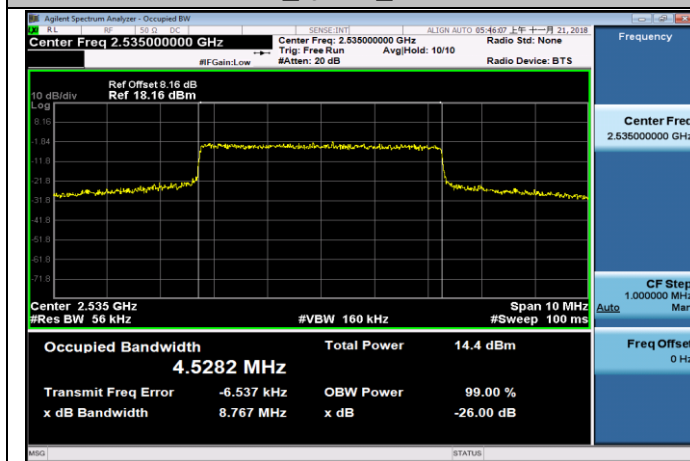
MCH_QPSK_25RB#0
