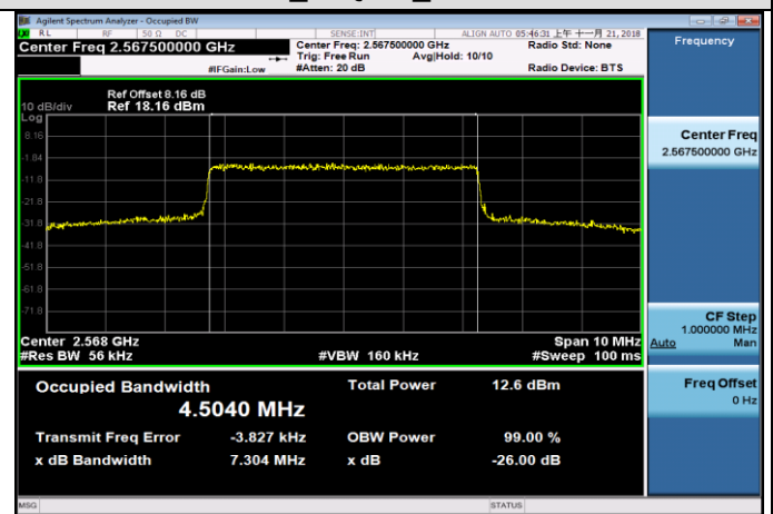
HCH_16QAM_25RB#0
