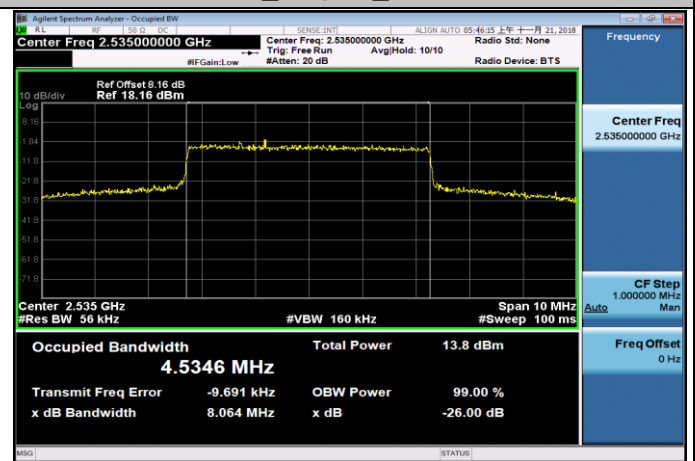
MCH_16QAM_25RB#0
