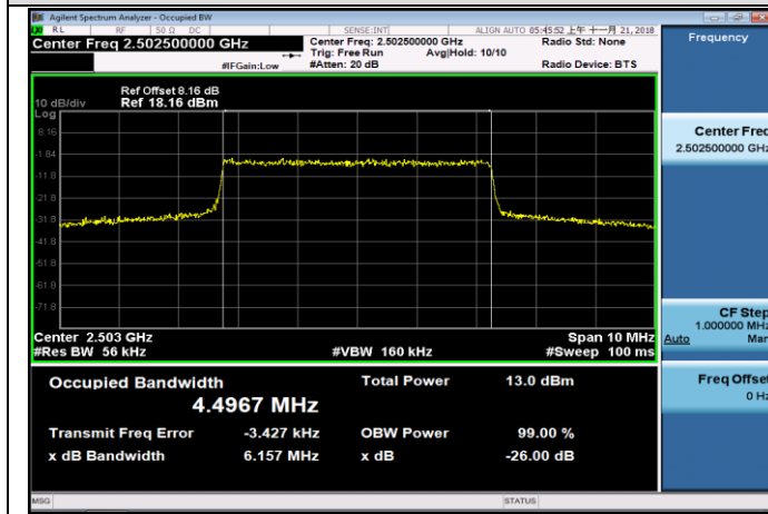
LCH_QPSK_25RB#0
