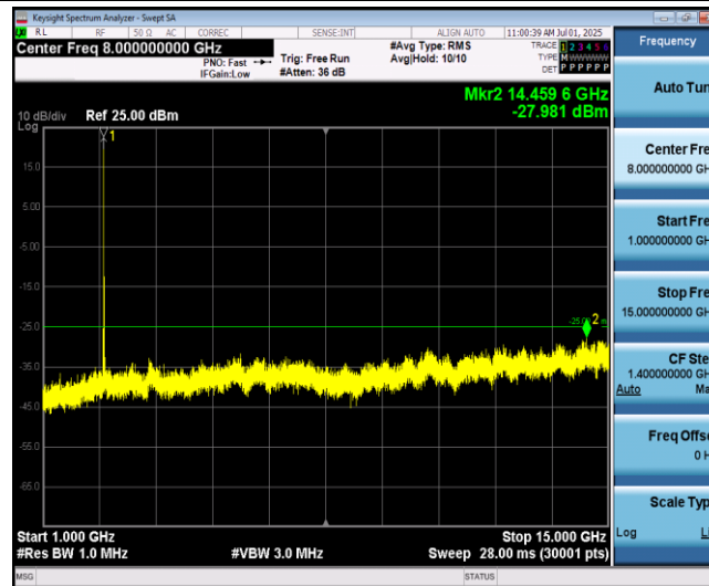
Band7-20MHz-16QAM-20850-1RB#0-Range2:1000~15000MHz
