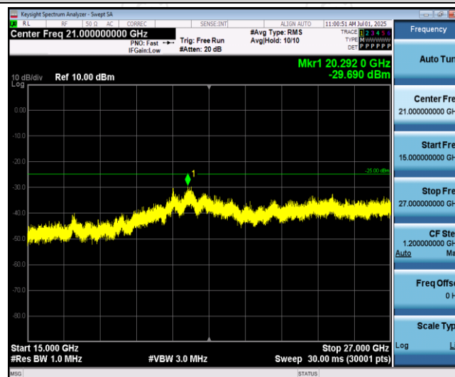
Band7-20MHz-16QAM-20850-1RB#0-Range3:15000~27000MHz
