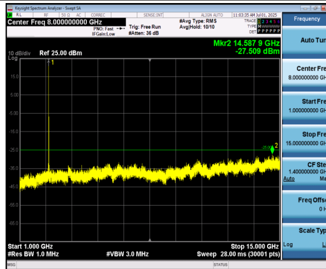
Band7-20MHz-16QAM-21350-1RB#0-Range2:1000~15000MHz
