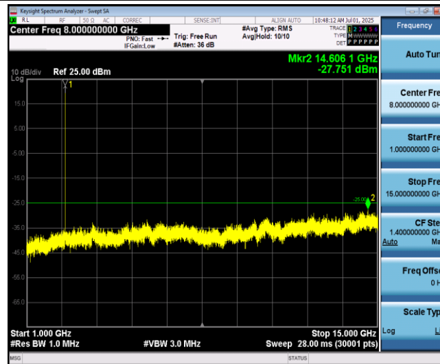
Band7-5MHz-QPSK-21100-1RB#0-Range2:1000~15000MHz
