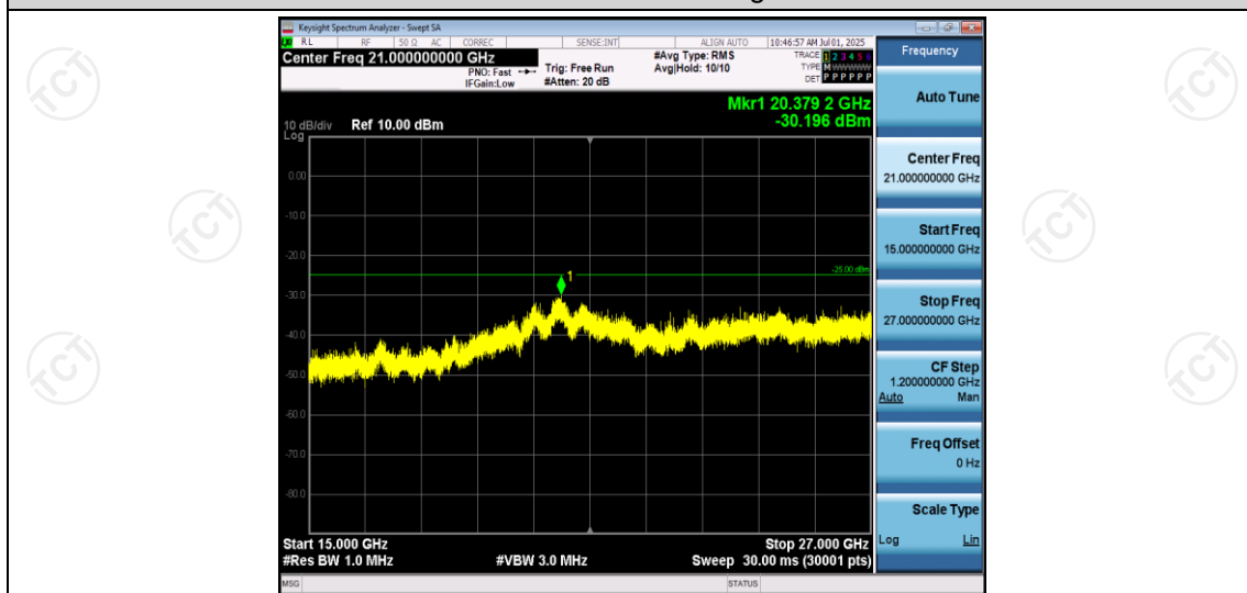
Band7-5MHz-QPSK-20775-1RB#0-Range3:15000~27000MHz
