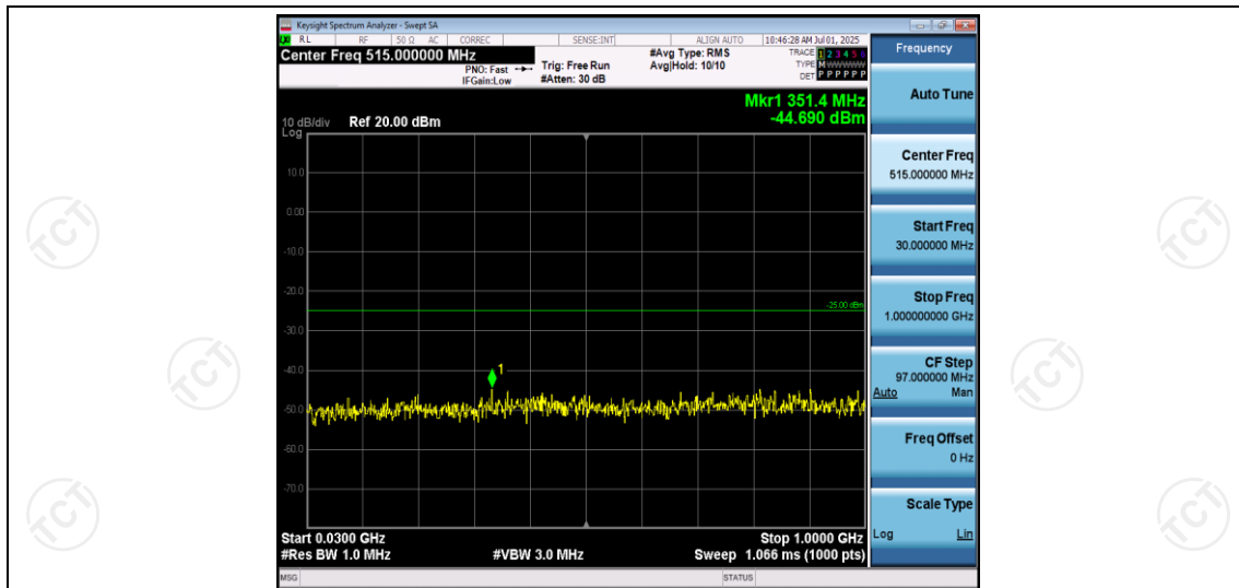
Band7-5MHz-QPSK-20775-1RB#0-Range1:30~1000MHz
