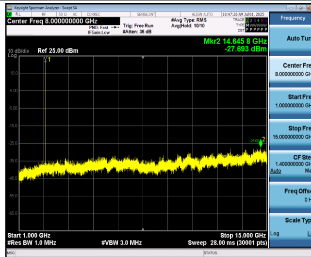
Band7-5MHz-16QAM-20775-1RB#0-Range2:1000~15000MHz
