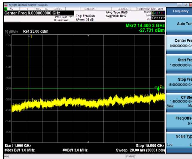
Band7-5MHz-QPSK-21425-1RB#0-Range2:1000~15000MHz
