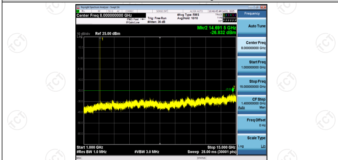
Band7-5MHz-QPSK-20775-1RB#0-Range2:1000~15000MHz
