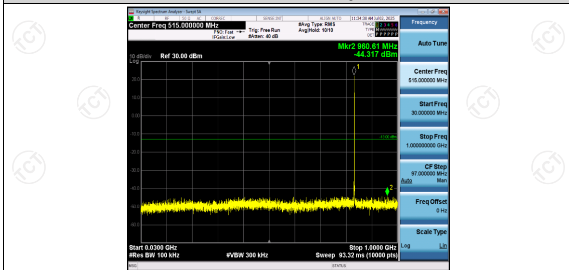
Band5-1.4MHz-QPSK-20525-1RB#0-Range1:30~1000MHz
