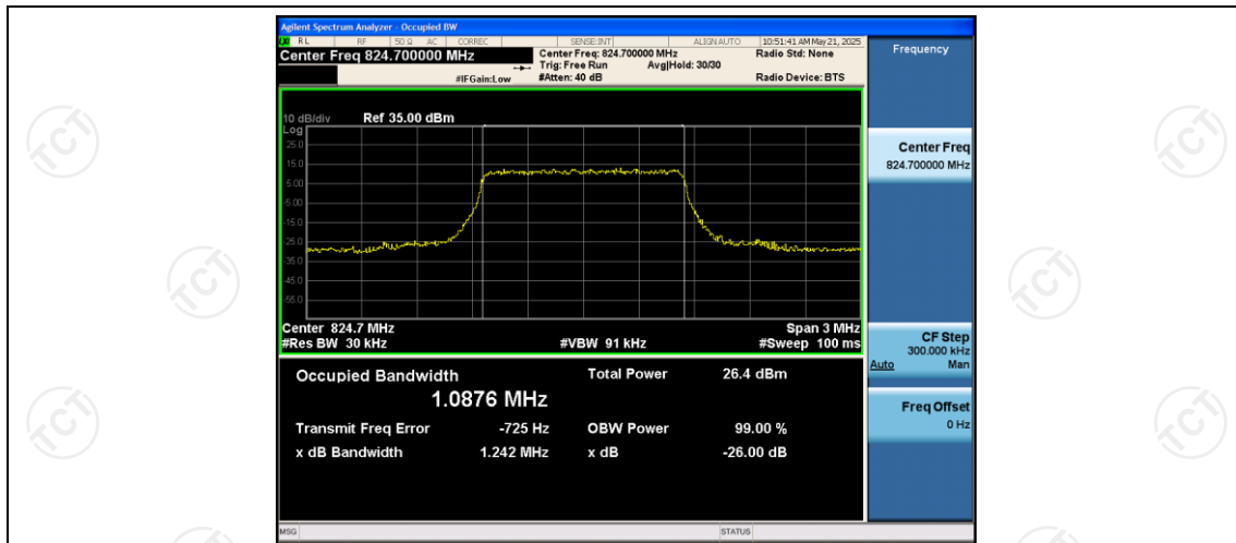
Band5-1.4MHz-QPSK-20407-6RB#0
