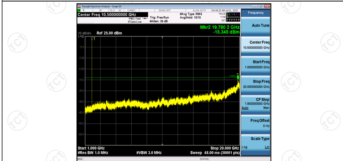
Band2-1.4MHz-QPSK-18607-1RB#0-Range2:1000~20000MHz
