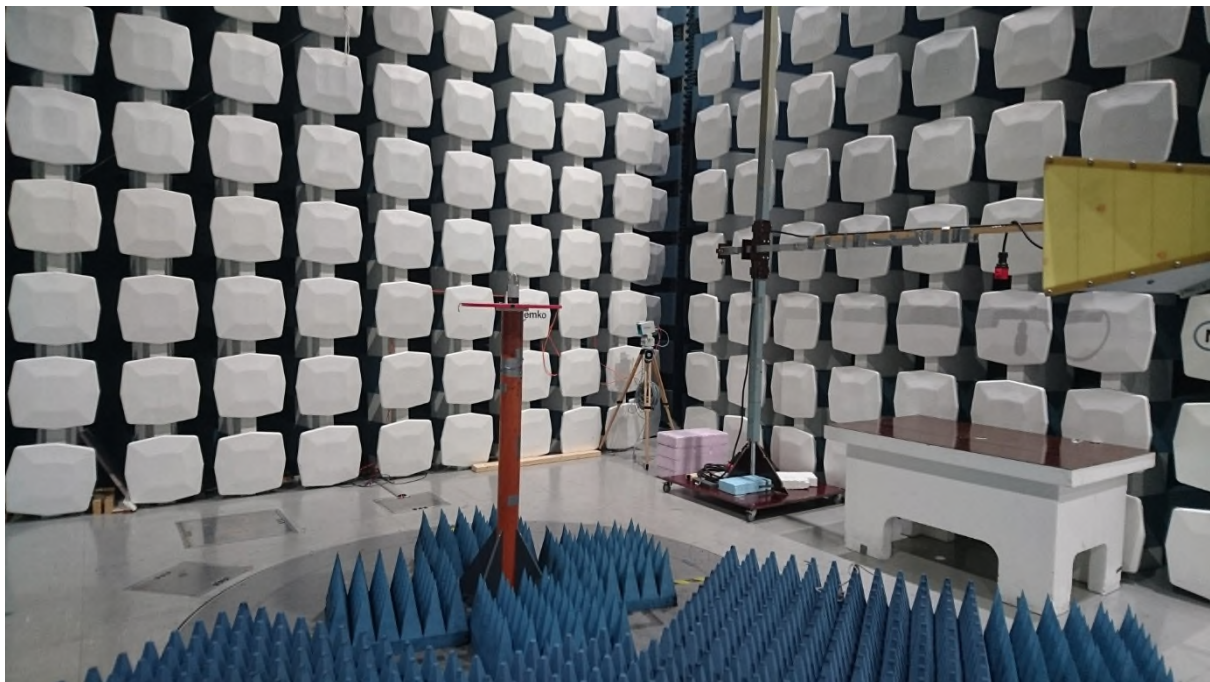
Radiated emissions 1 - 3GHz
