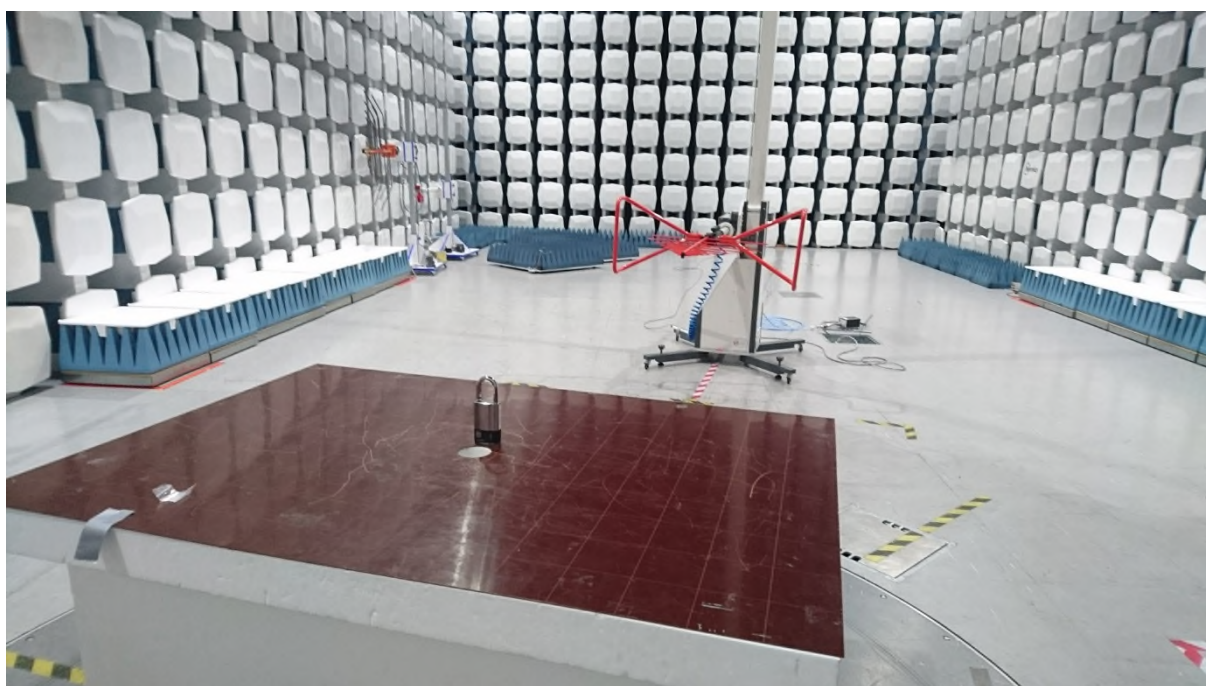
Radiated emission 30 - 1000 MHz
