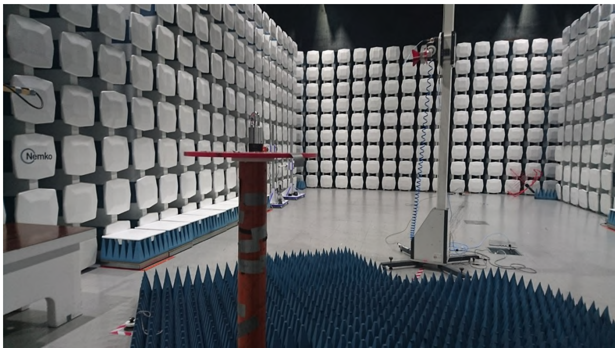
Radiated emissions 3 - 18GHz
