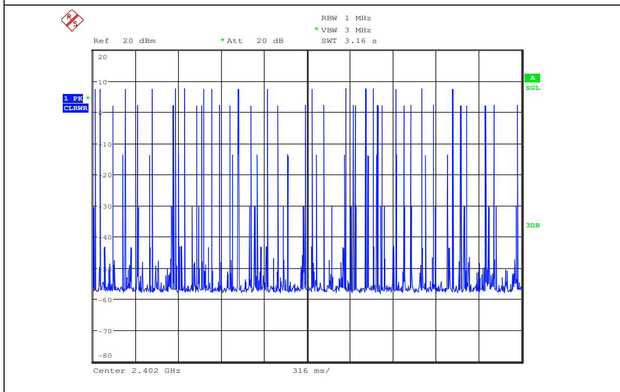
Dwell Time_DH5_2402
