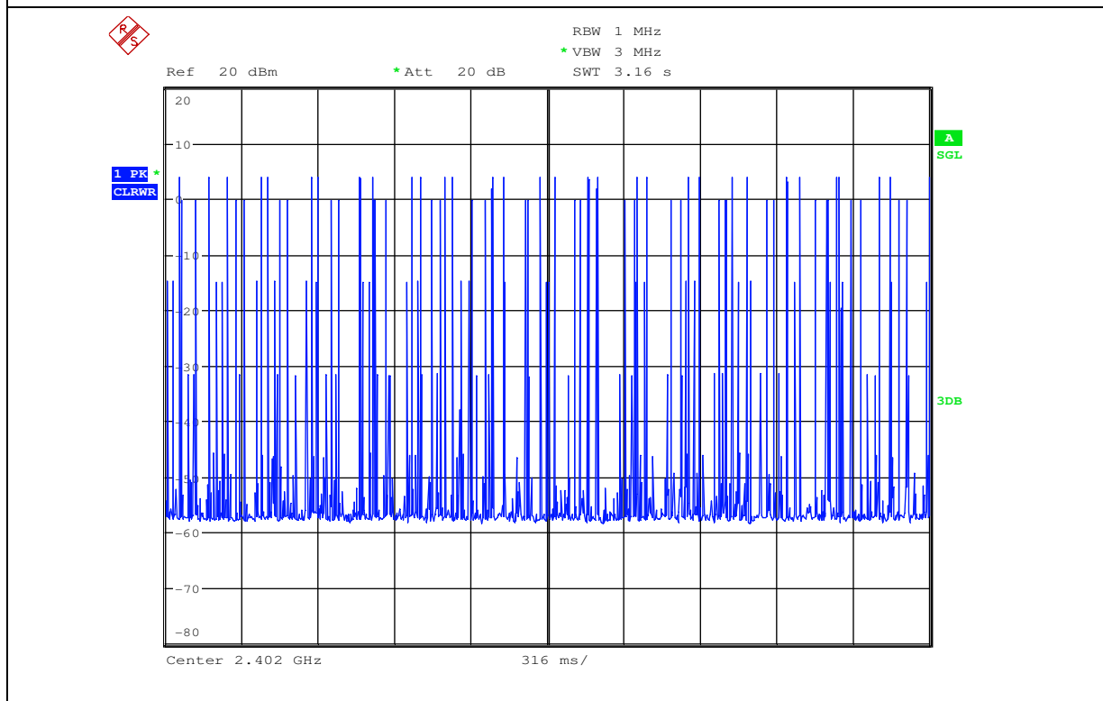
Dwell Time_2DH3_2402
