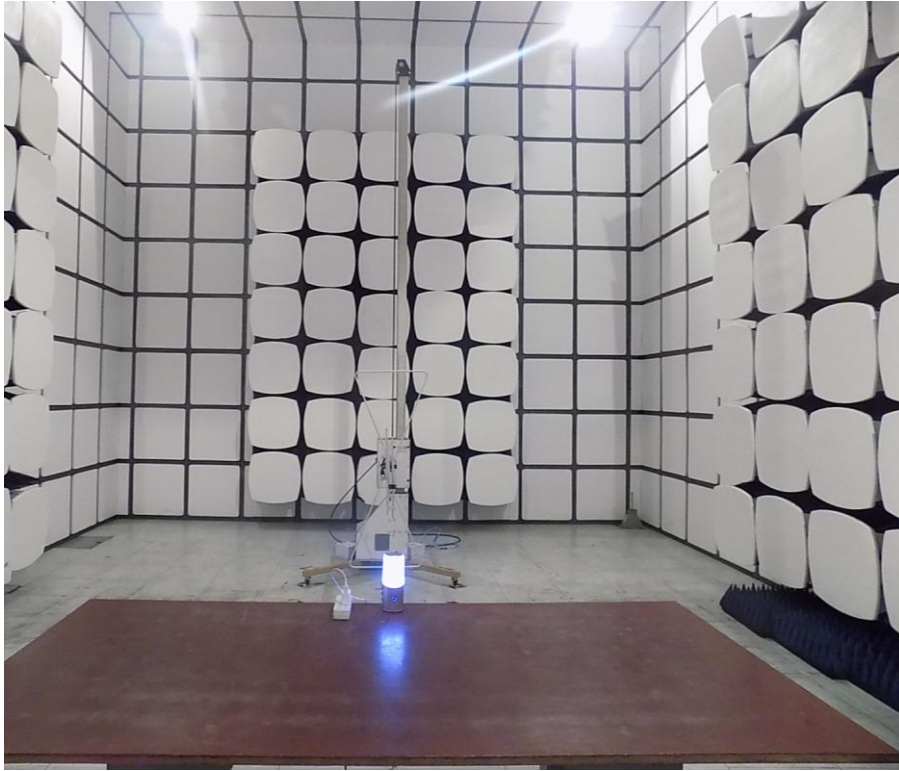
Photos of Radiated emission
