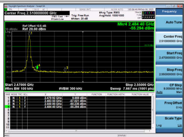
2DH5-Ant1-2480-PASS
