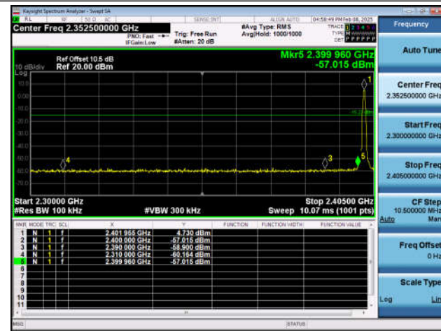
DH5-Ant1-Hop_2402-PASS
