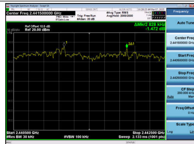
3DH5-Ant1-Hop-PASS
