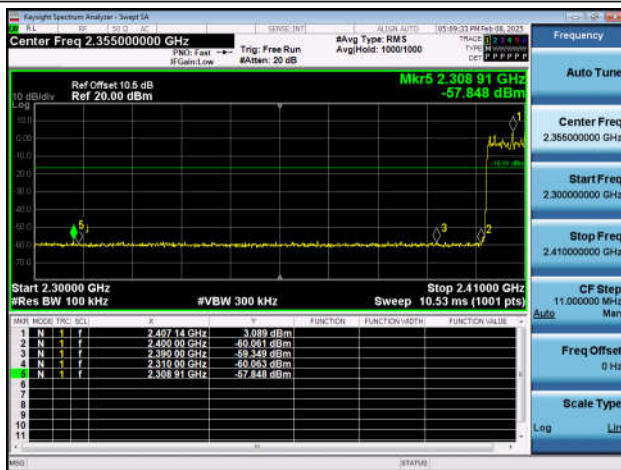
3DH5-Ant1-2402-PASS
