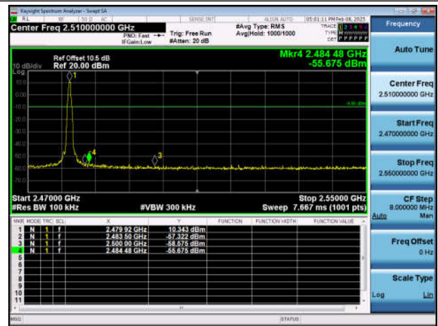
DH5-Ant1-Hop_2480-PASS
