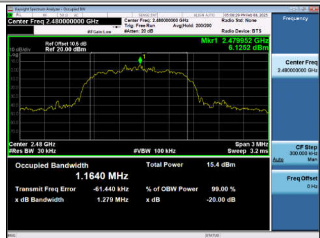
2DH5-Ant1-2480
