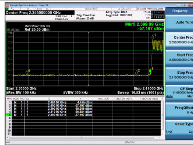
2DH5-Ant1-2402-PASS
