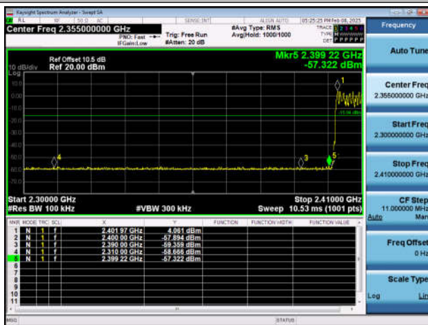
3DH5-Ant1-Hop_2402-PASS
