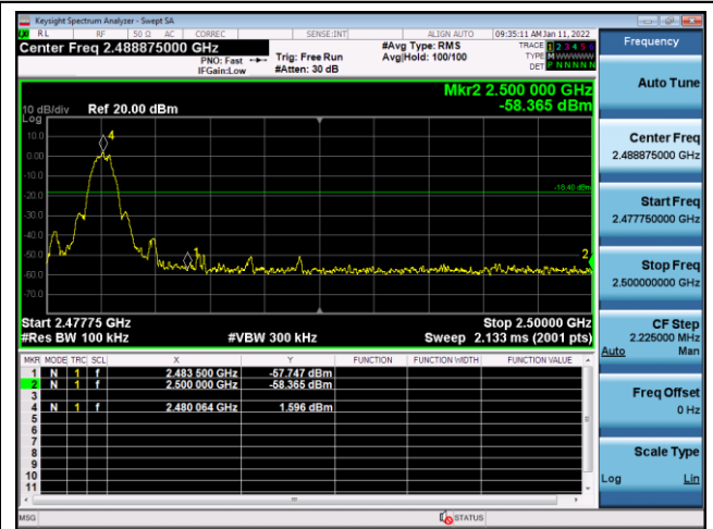
Channel 39 / 2480 MHz
