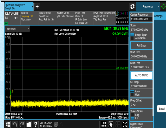
11N40ISO-Ant1-2452-30-1000-PASS
