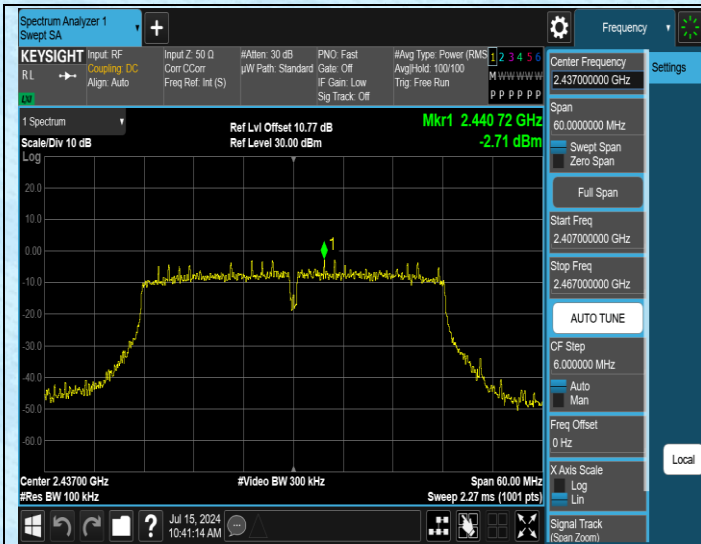
11N40ISO-Ant1-2437-0-Reference-PASS
