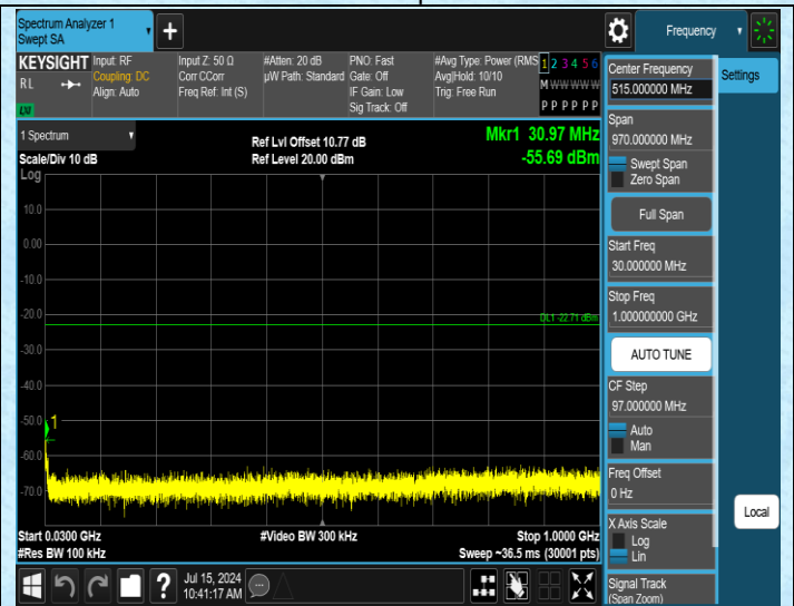
11N40ISO-Ant1-2437-30-1000-PASS
