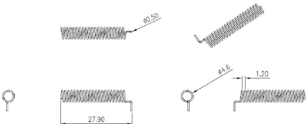
Antenna dimension design
