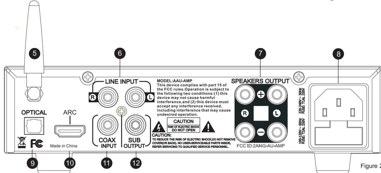
Figure 2. Rear Panel
