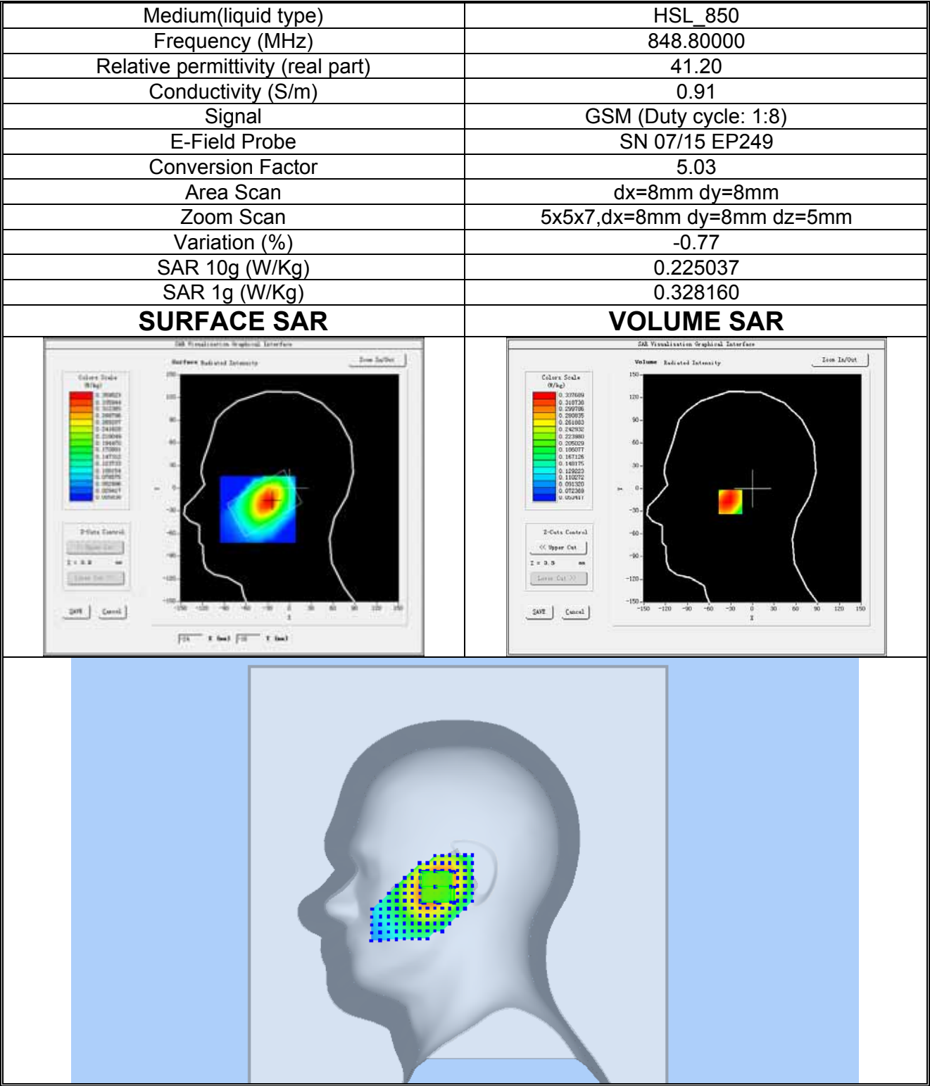
Plot 2: GSM850MHz, High channel (Right Head , Tilt) Product Description: Mobile phone Test Date:2017-09-21
