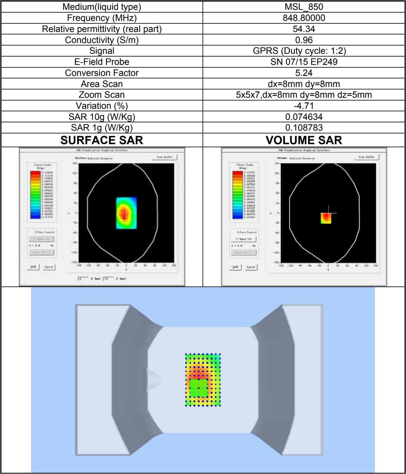
Plot 7: GPRS850MHz, High channel(Body-worn, Right side) Product Description: Mobile phone Test Date: 2017-09-21
