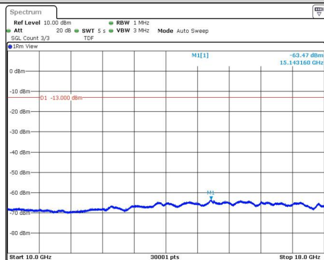
Band5-4132-3-10000~18000MHz
