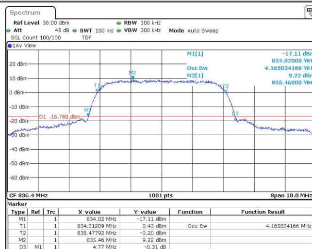
Band5-4182-2-4.77
