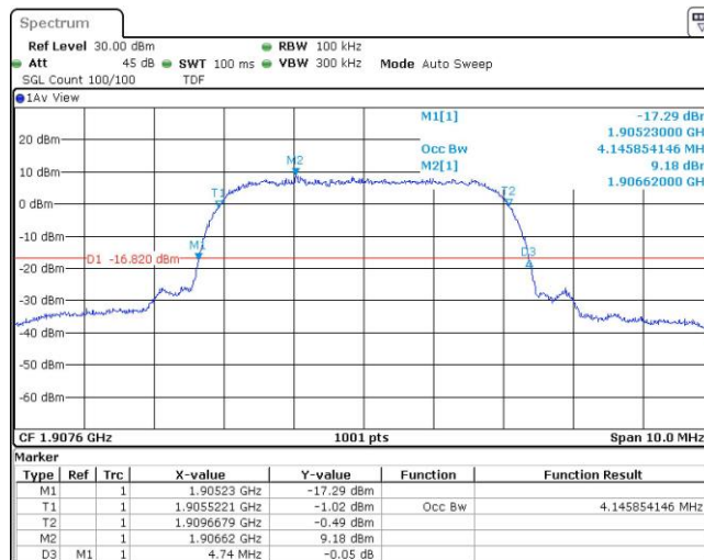
Band2-9538-4-4.74
