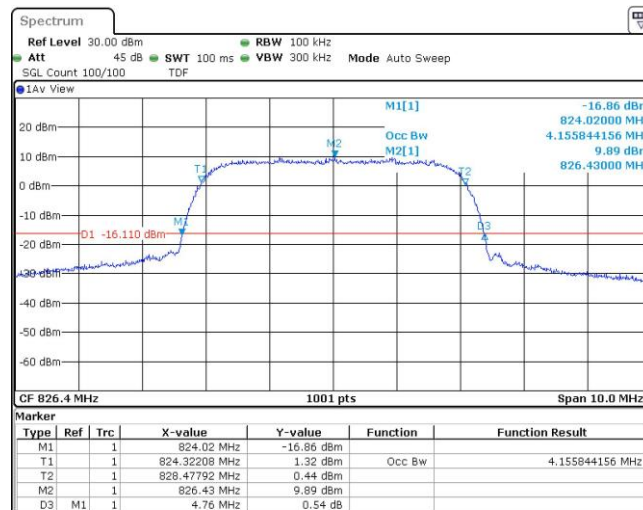
Band5-4182-1-4.77
