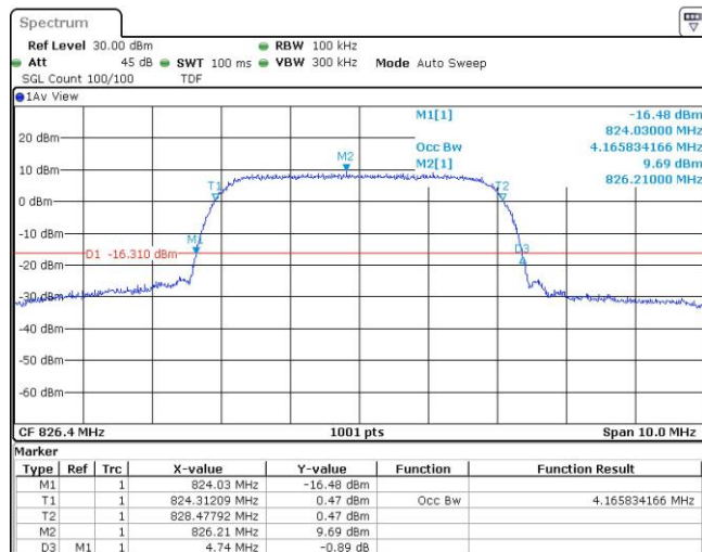
Band5-4132-2-4.75
