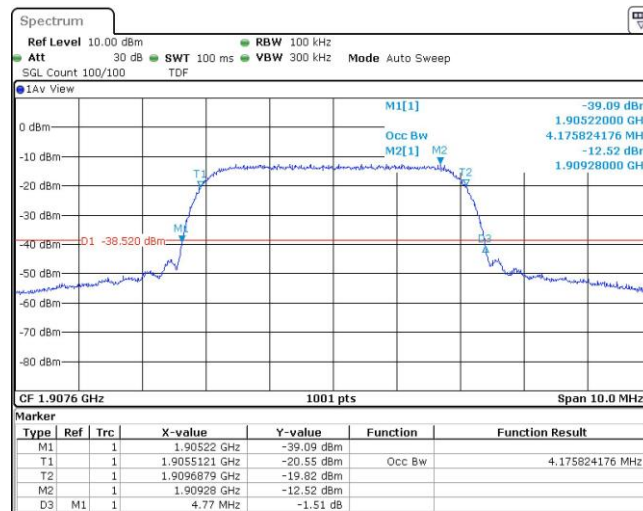
Band2-9538-4-4.76
