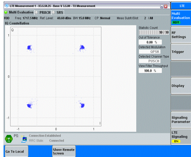
Band4-15MHz-QPSK-20175-38RB#0
