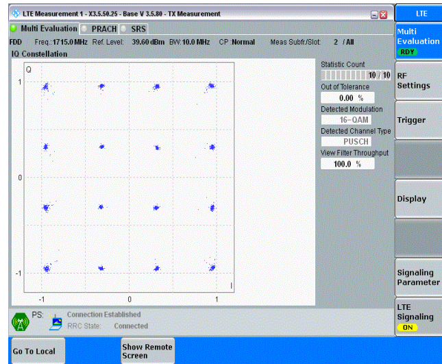
Band4-10MHz-16QAM-20175-25RB#0
