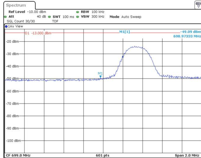
Band12-5MHz-16QAM-23035-25RB#0
