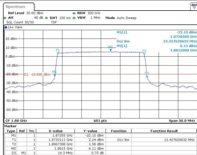
Band2-15MHz-16QAM-18900-38RB#0
