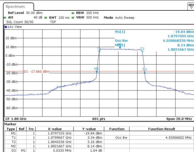
Band2-10MHz-16QAM-19150-25RB#25
