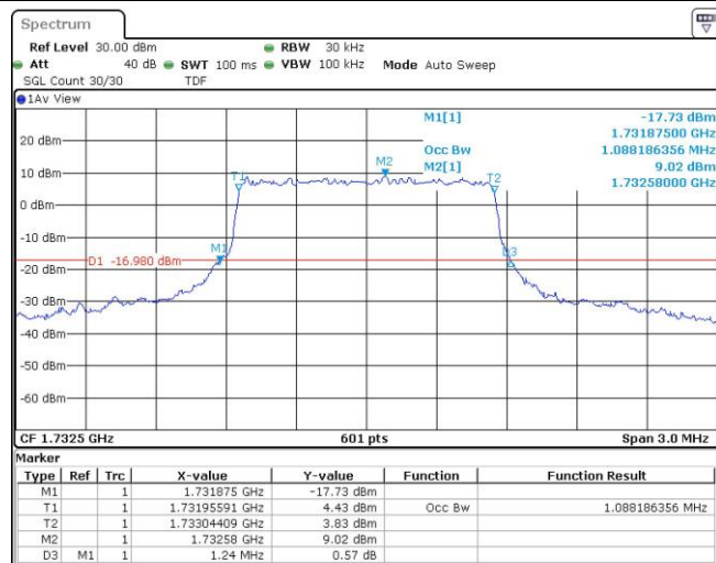
Band4-1.4MHz-QPSK-20175-6RB#0
