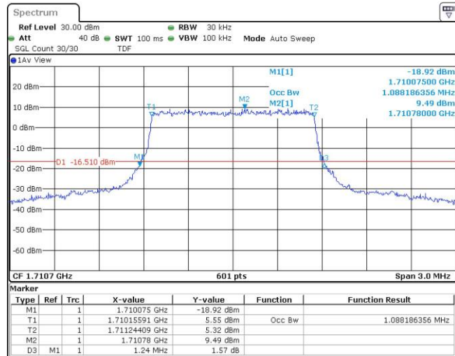
Band4-1.4MHz-QPSK-20175-6RB#0
