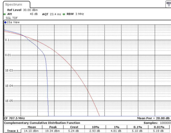
Band12-5MHz-16QAM-23095-25RB#0
