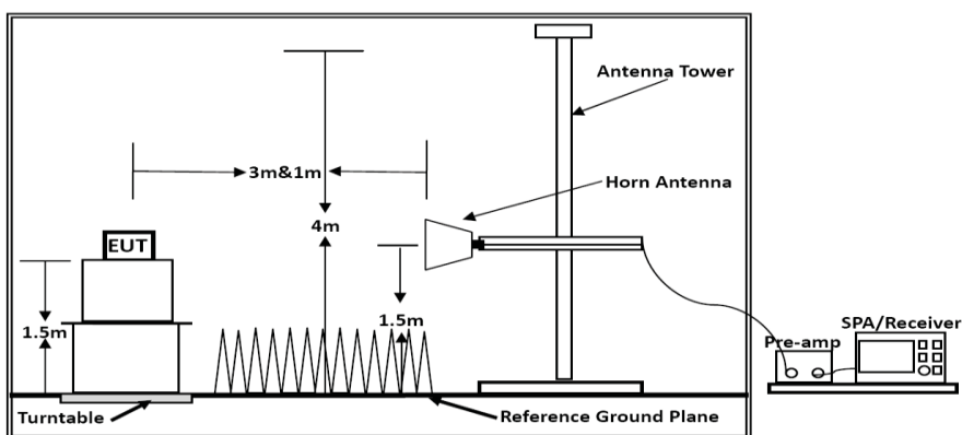
Above 1GHz
